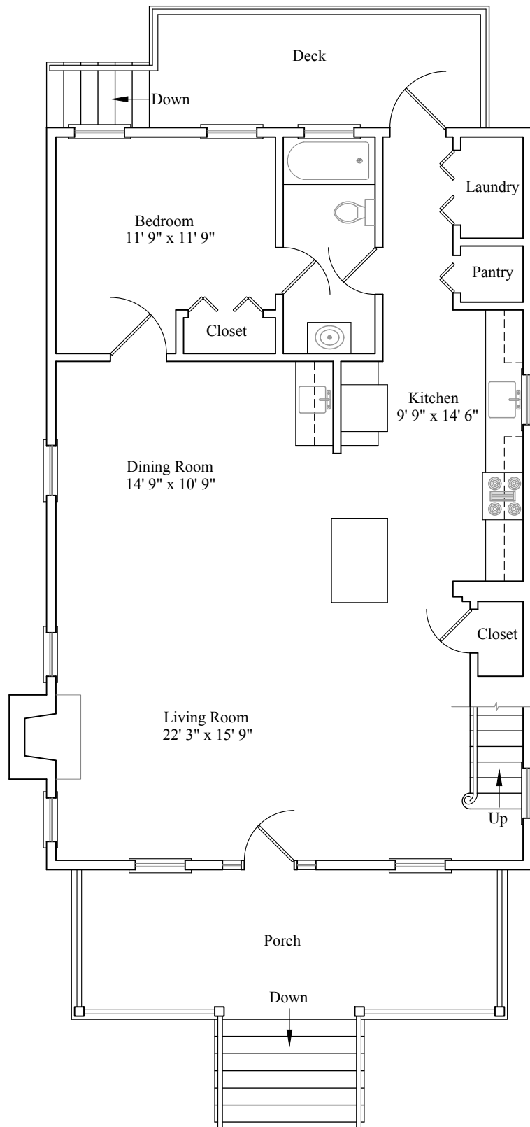
← Bennett Street → First Floor Plan
